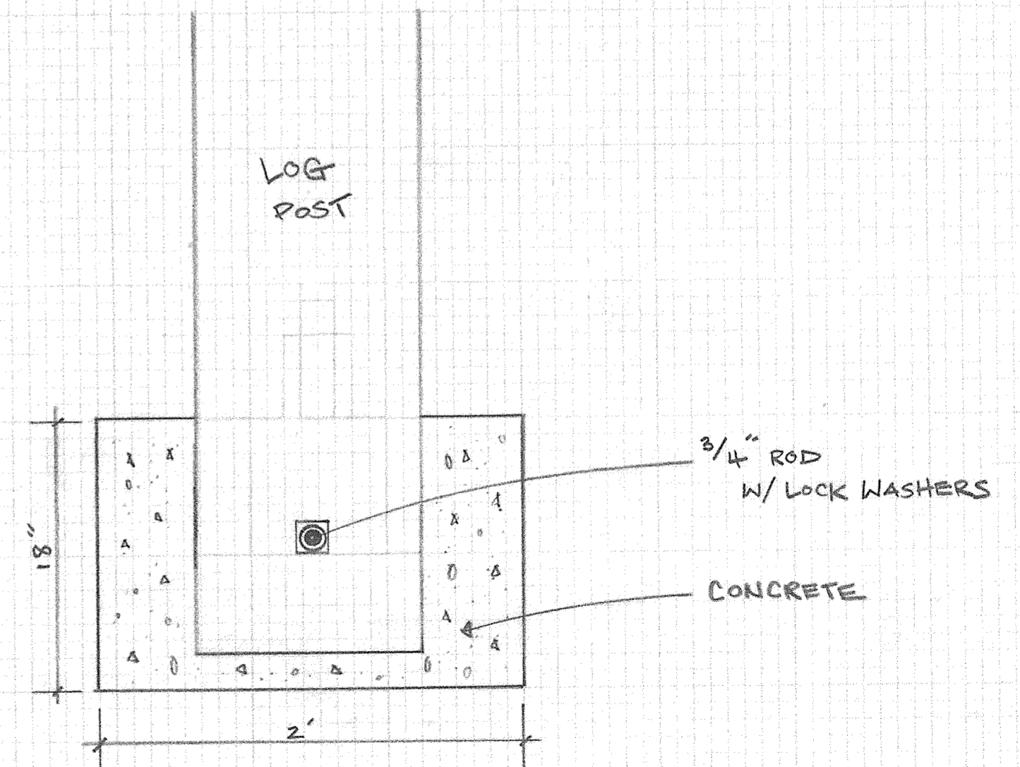
ALT. POST SUPPORT DETAIL
